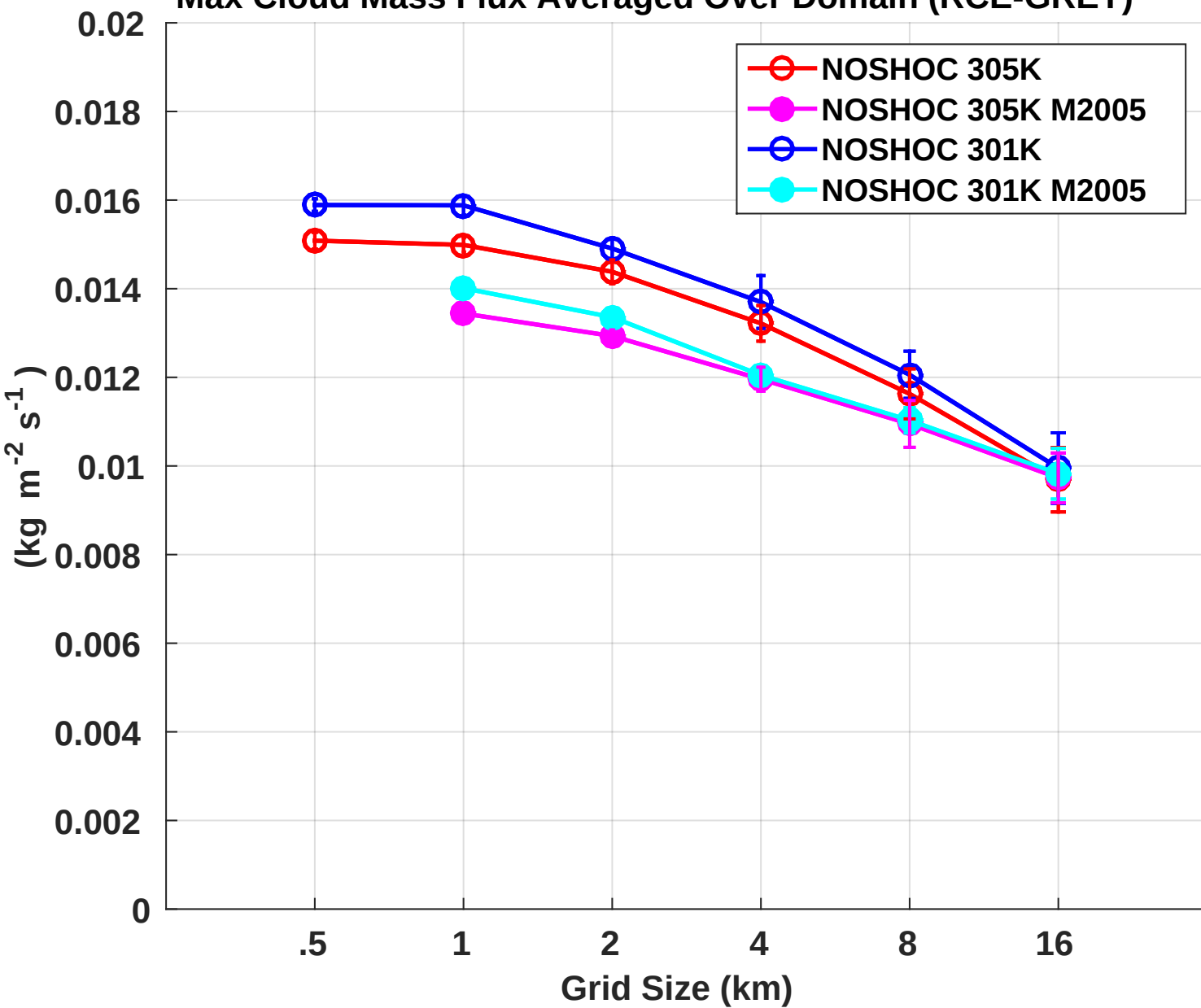
Max Cloud Mass Flux Averaged Over Domain (RCE-GREY)
