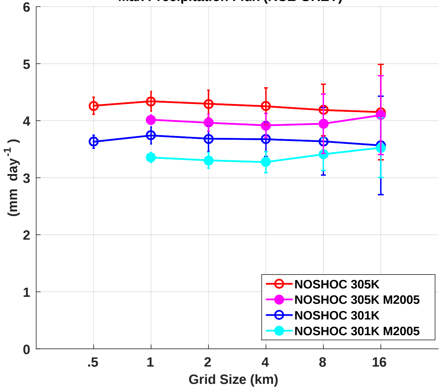
Max Precipitation Flux (RCE-GREY)
