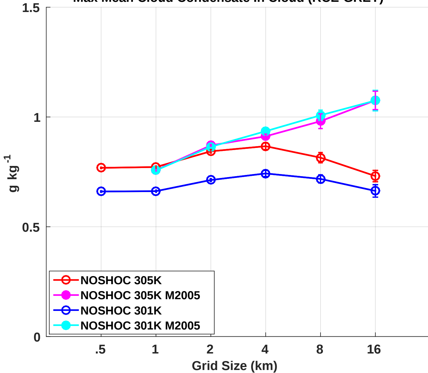
Max Mean Cloud Condensate In Cloud (RCE-GREY)
