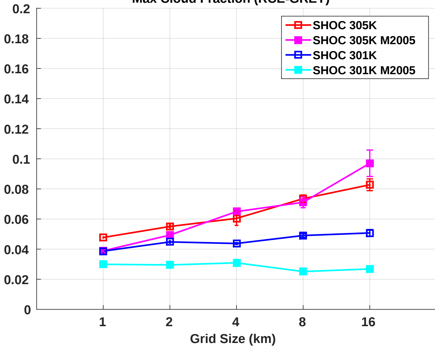
Max Cloud Fraction (RCE-GREY)
