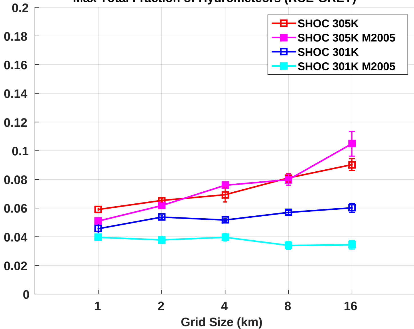
Max Total Fraction of Hydrometeors (RCE-GREY)
