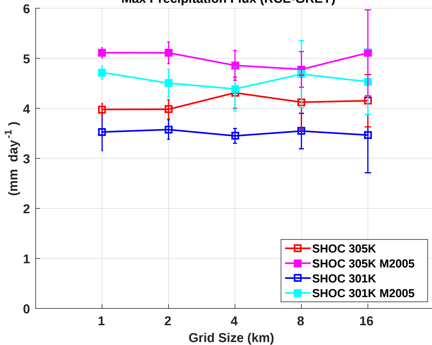
Max Precipitation Flux (RCE-GREY)
