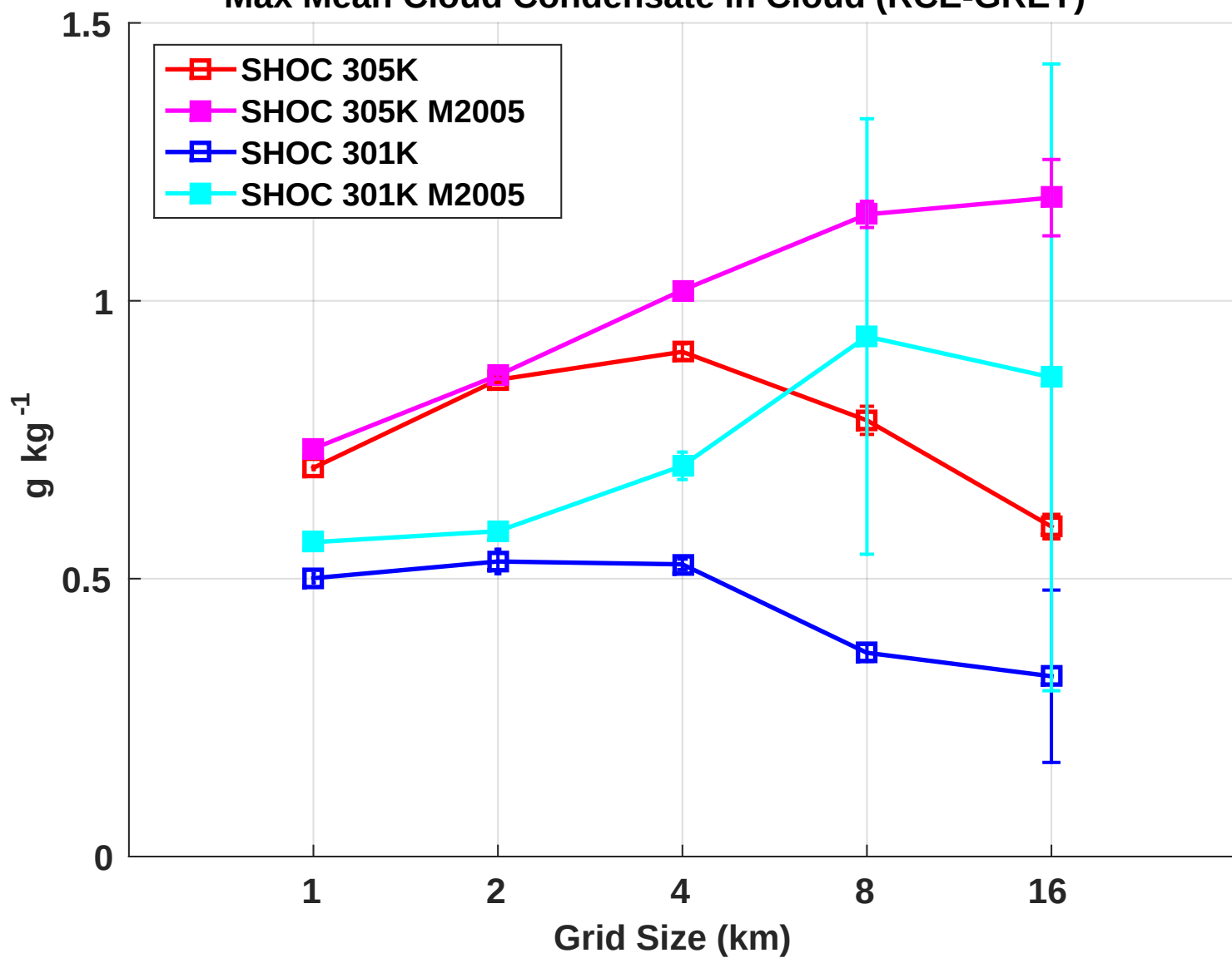
Max Mean Cloud Condensate in Cloud (RCE-GREY)
