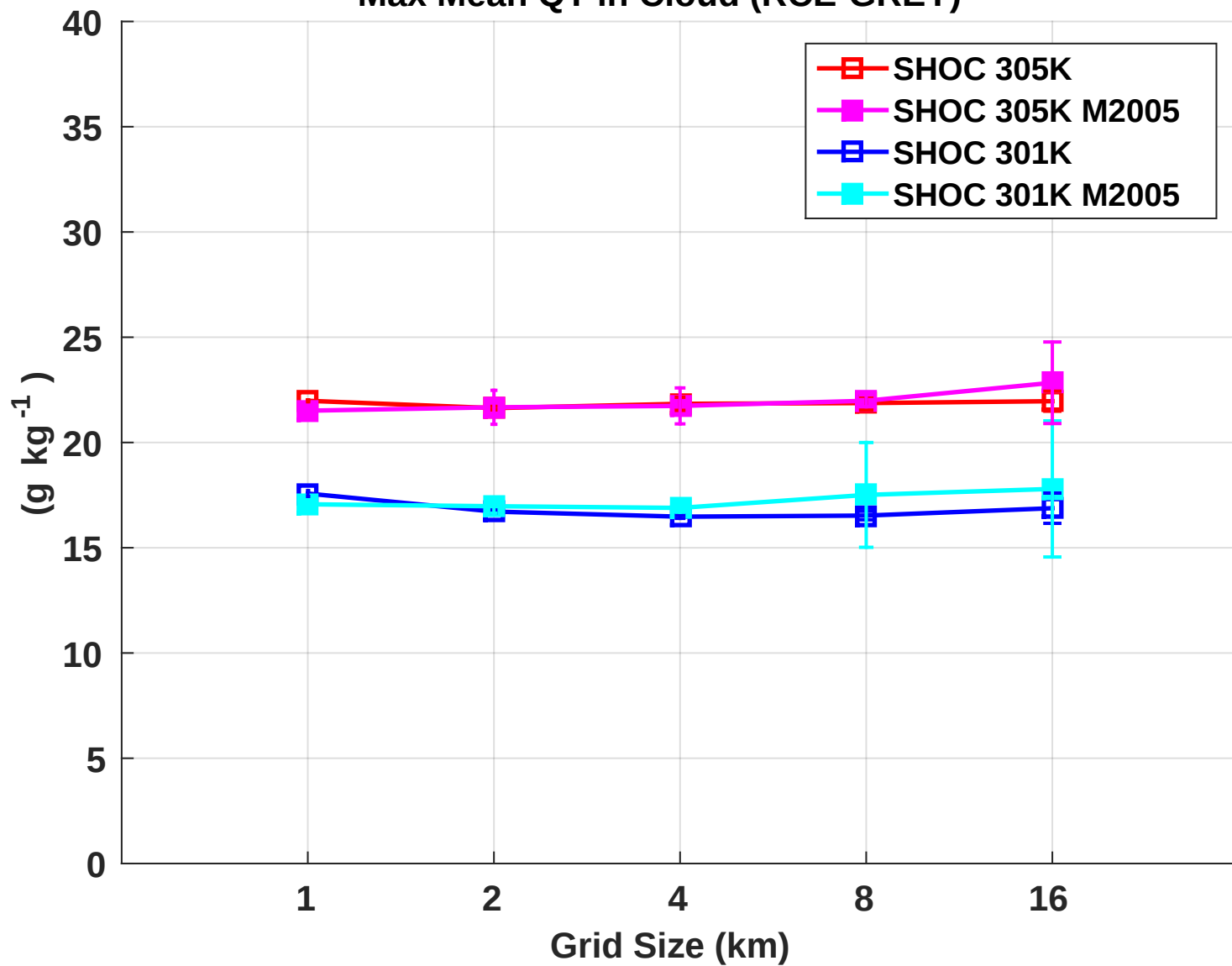
Max Mean QT in Cloud (RCE-GREY)
