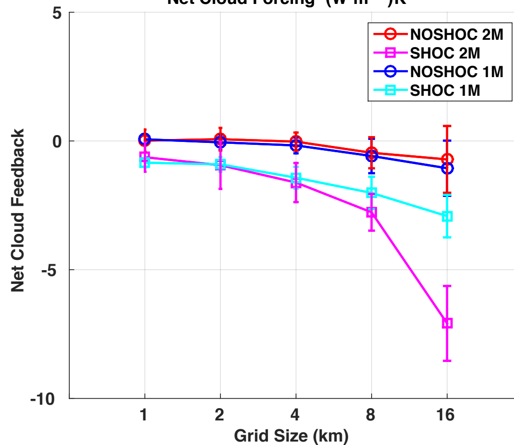
Net Cloud Forcing ( \text{W m}^{-2} \text{K}^{-1} )
