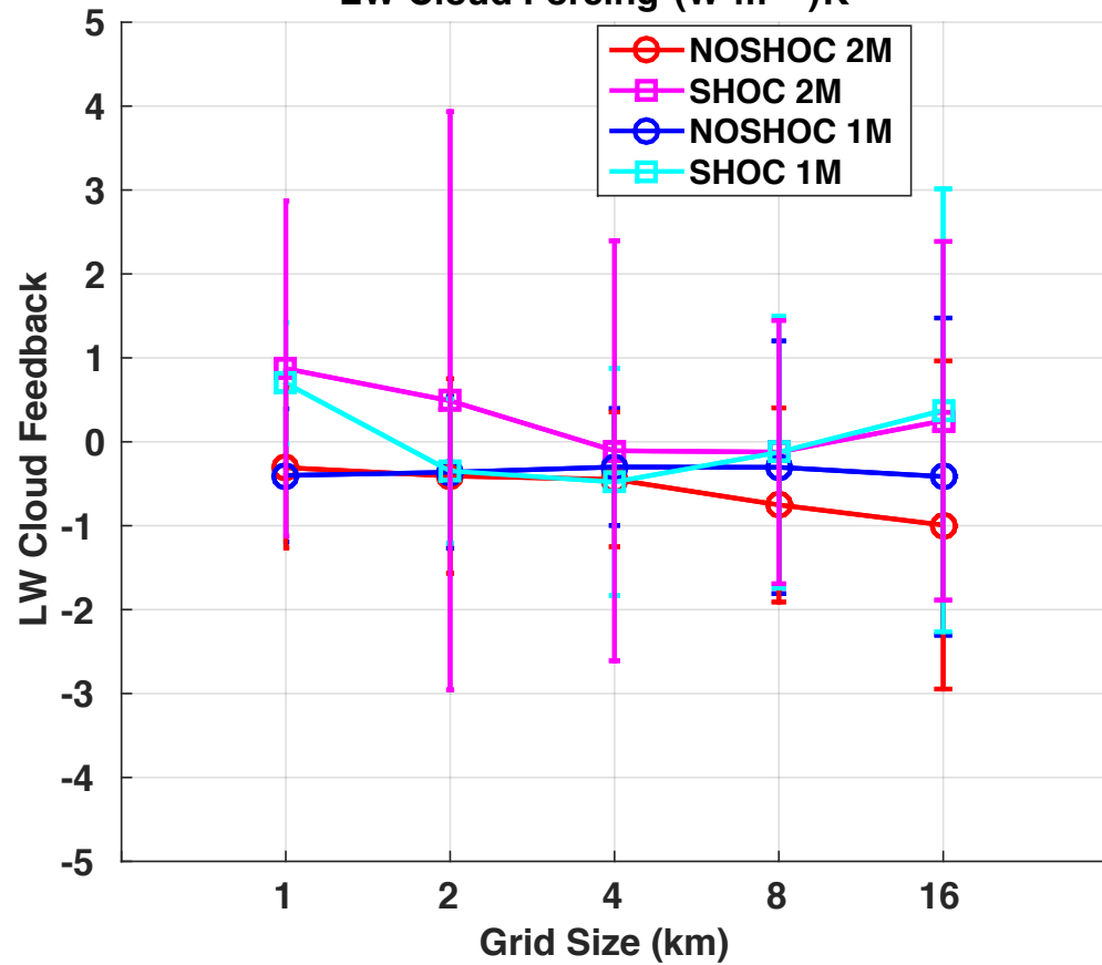
LW Cloud Forcing ( \text{W m}^{-2} \text{K}^{-1} )
