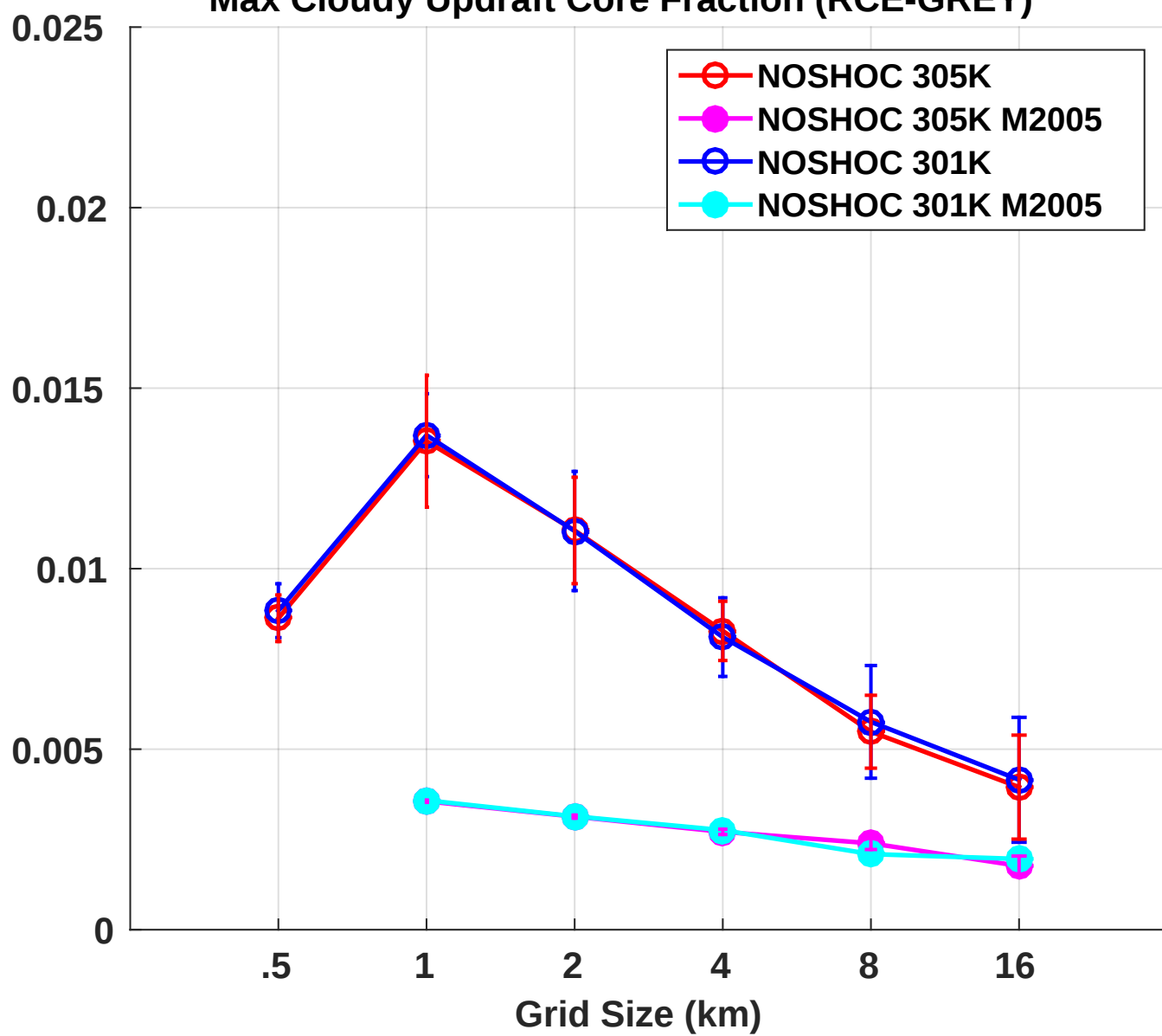
Max Cloudy Updraft Core Fraction (RCE-GREY)
