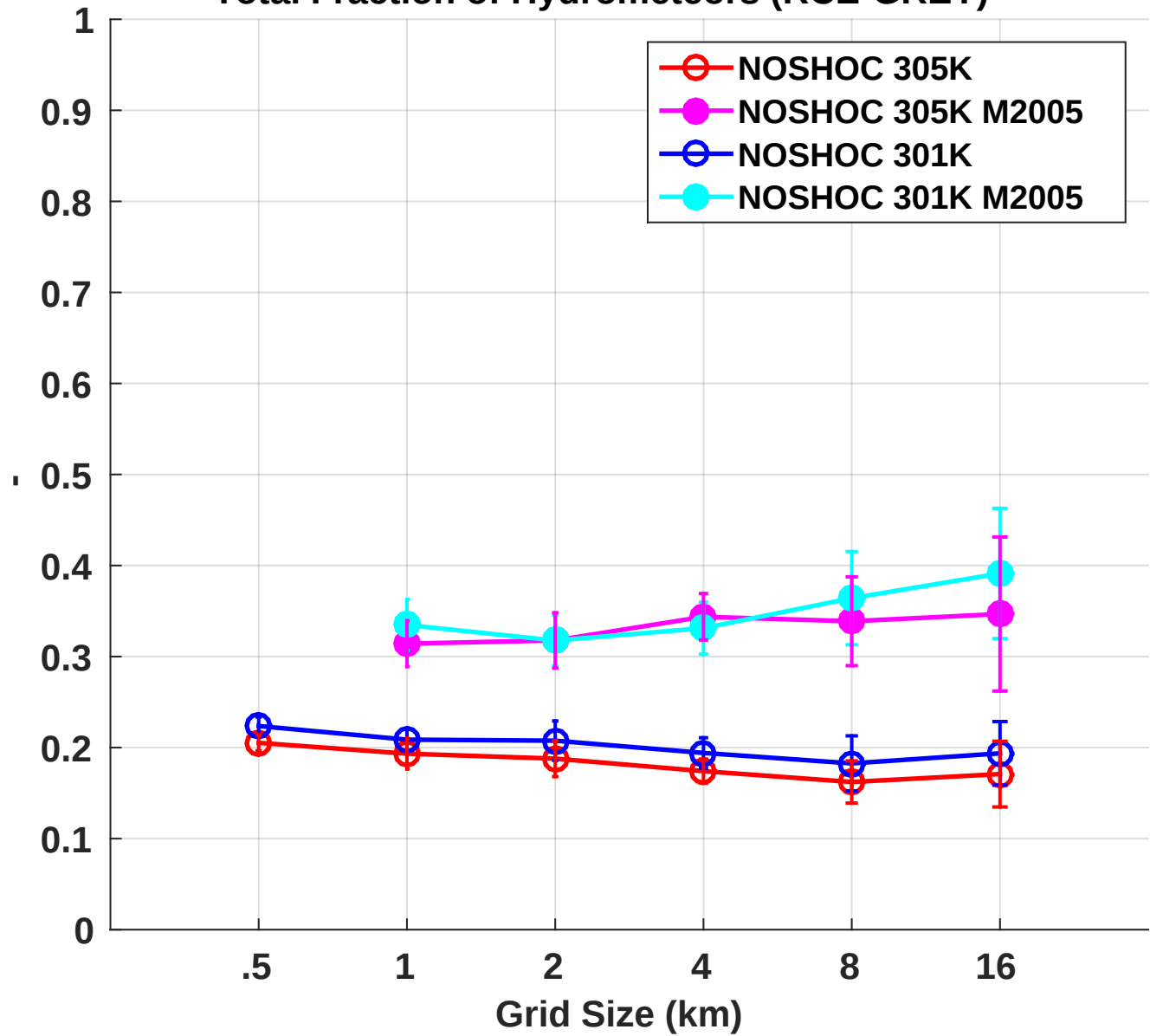
Total Fraction of Hydrometeors (RCE-GREY)
