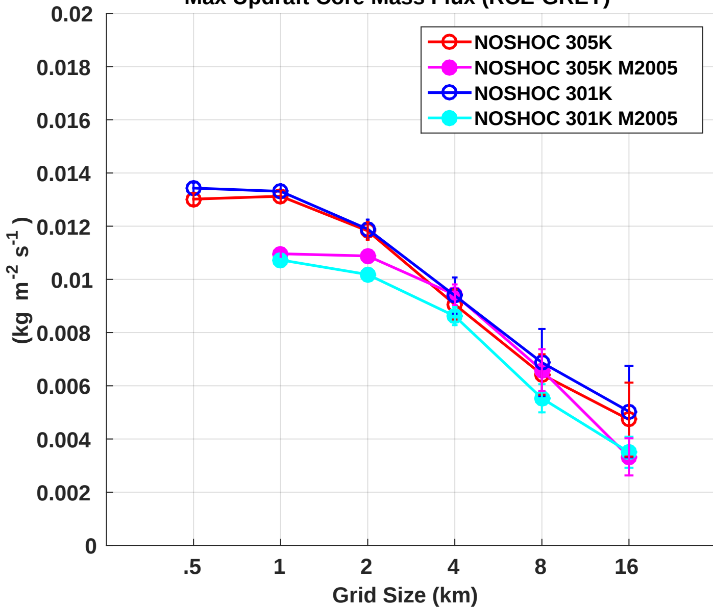
Max Updraft Core Mass Flux (RCE-GREY)
