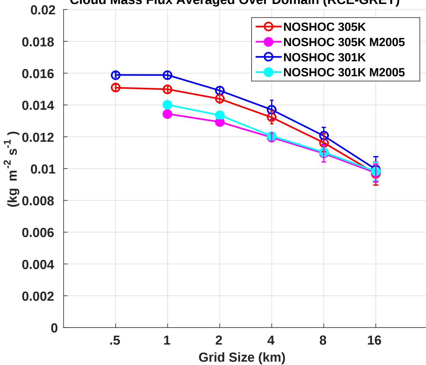
Cloud Mass Flux Averaged Over Domain (RCE-GREY)
