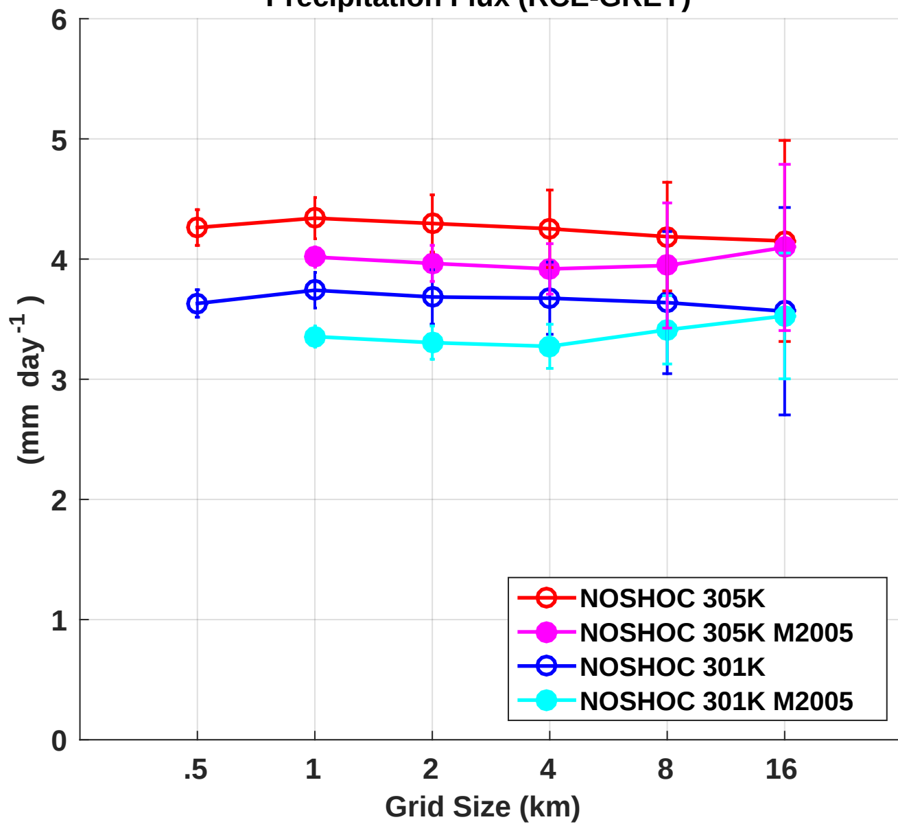
Precipitation Flux (RCE-GREY)
