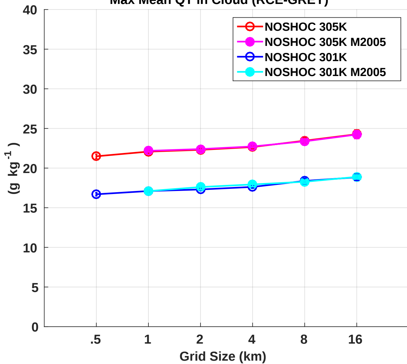
Max Mean QT in Cloud (RCE-GREY)
