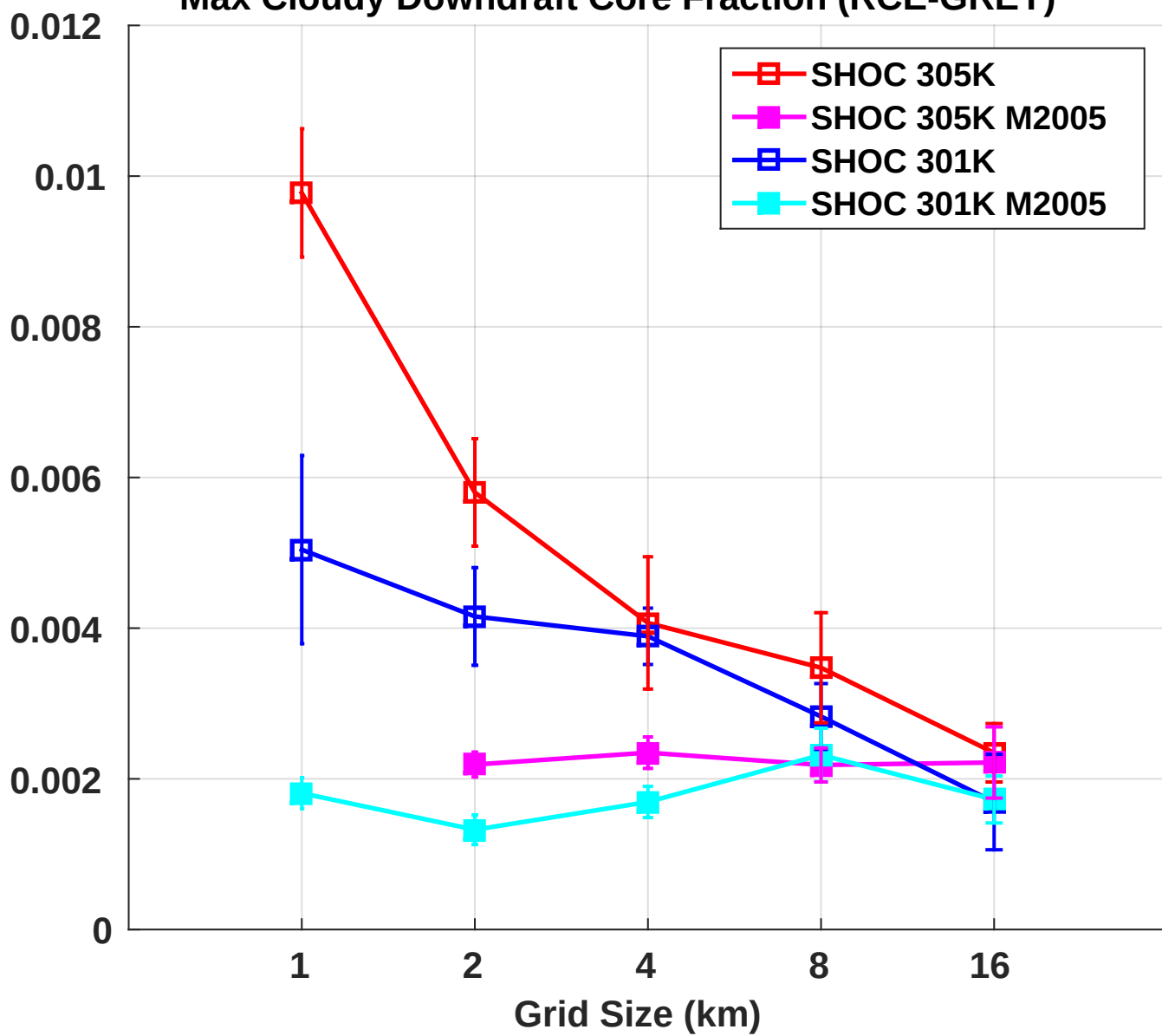
Max Cloudy Downdraft Core Fraction (RCE-GREY)
