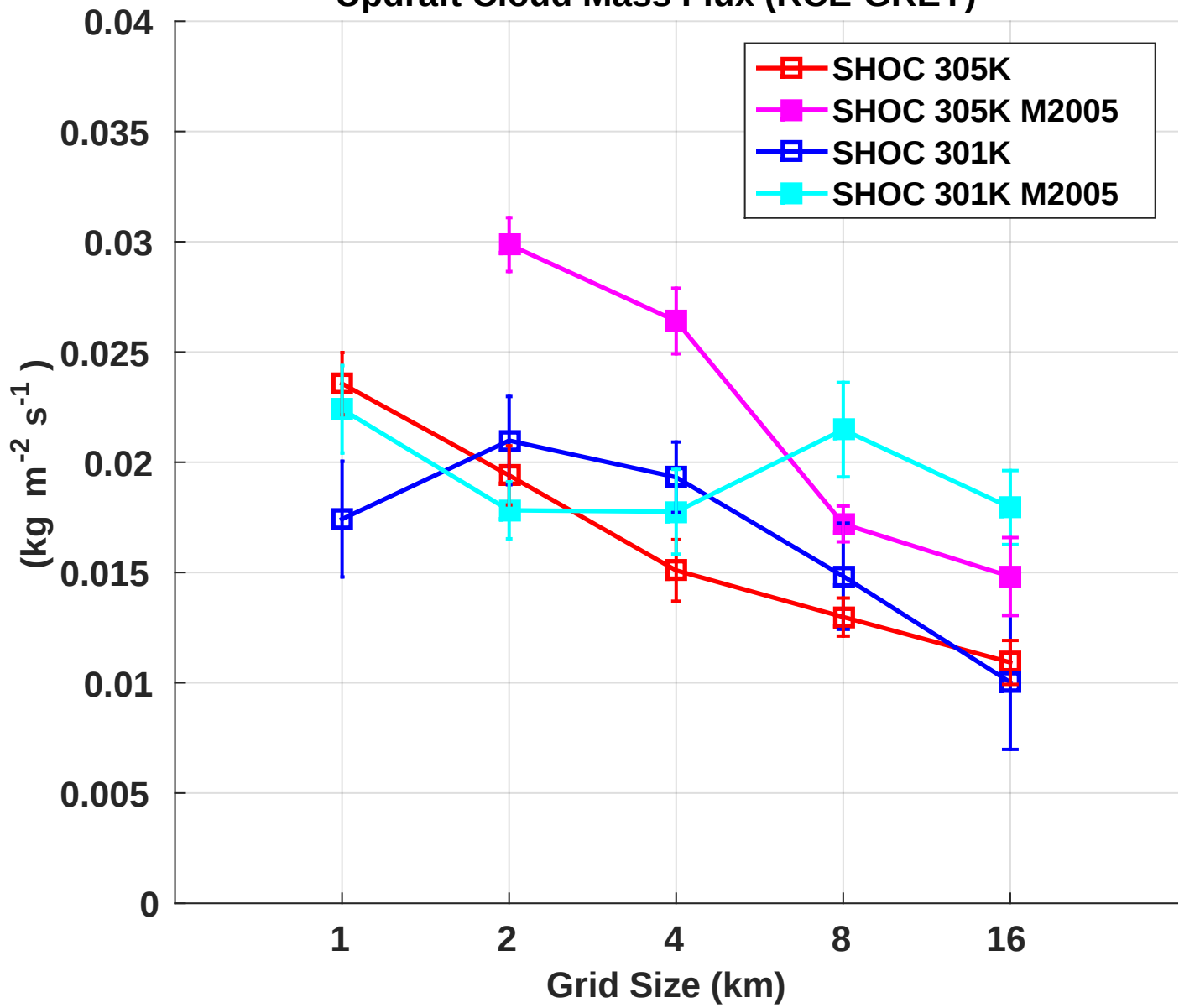
Updraft Cloud Mass Flux (RCE-GREY)
