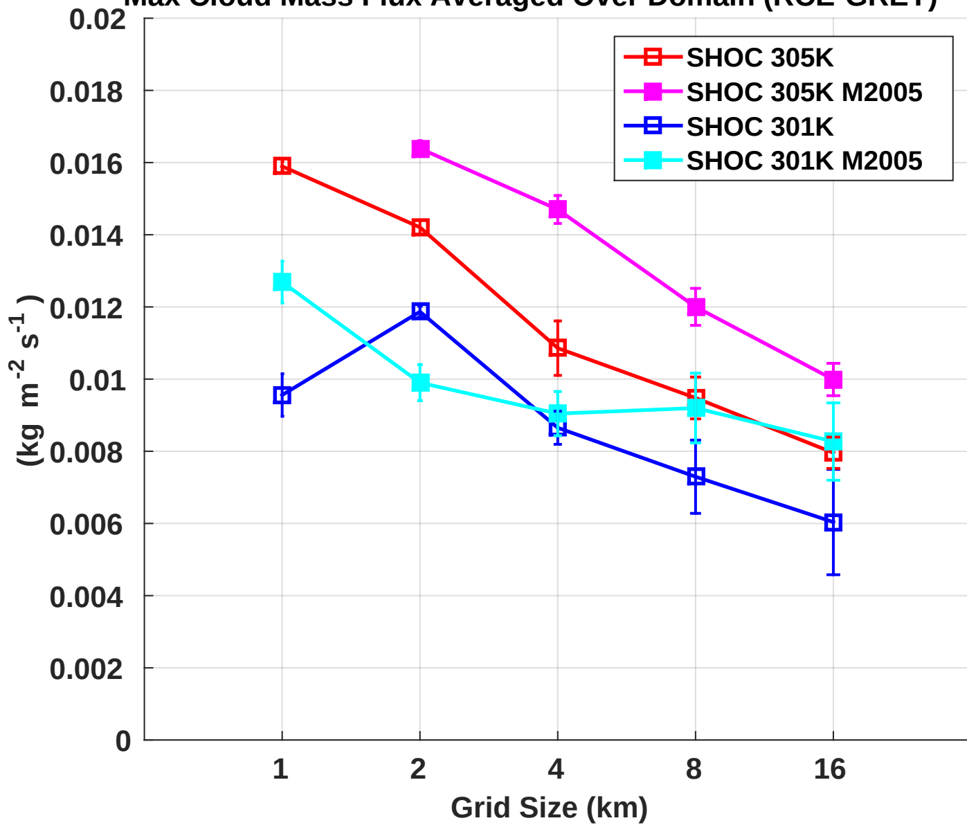
Max Cloud Mass Flux Averaged Over Domain (RCE-GREY)
