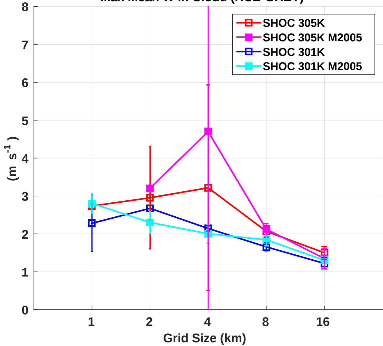
Max Mean W in Cloud (RCE-GREY)
