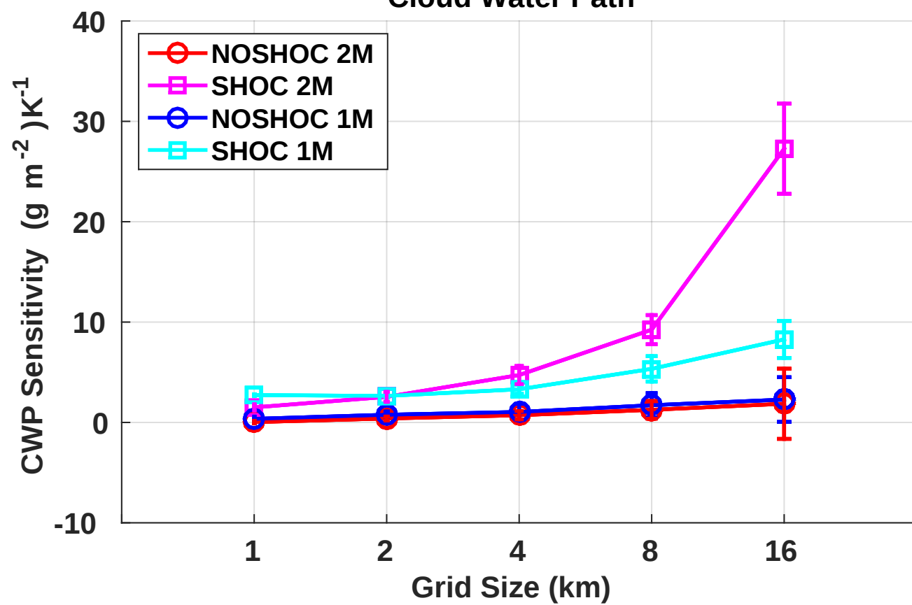
Cloud Water Path
