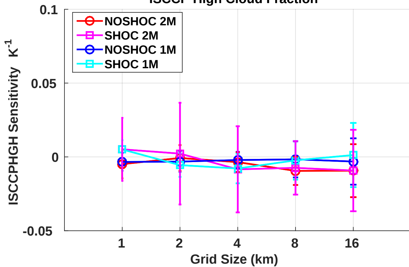
ISCCP High Cloud Fraction
