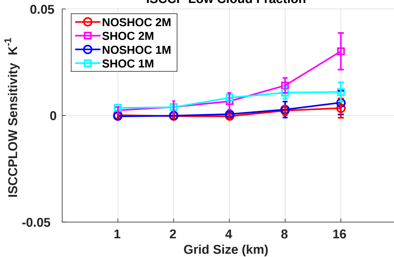
ISCCP Low Cloud Fraction
