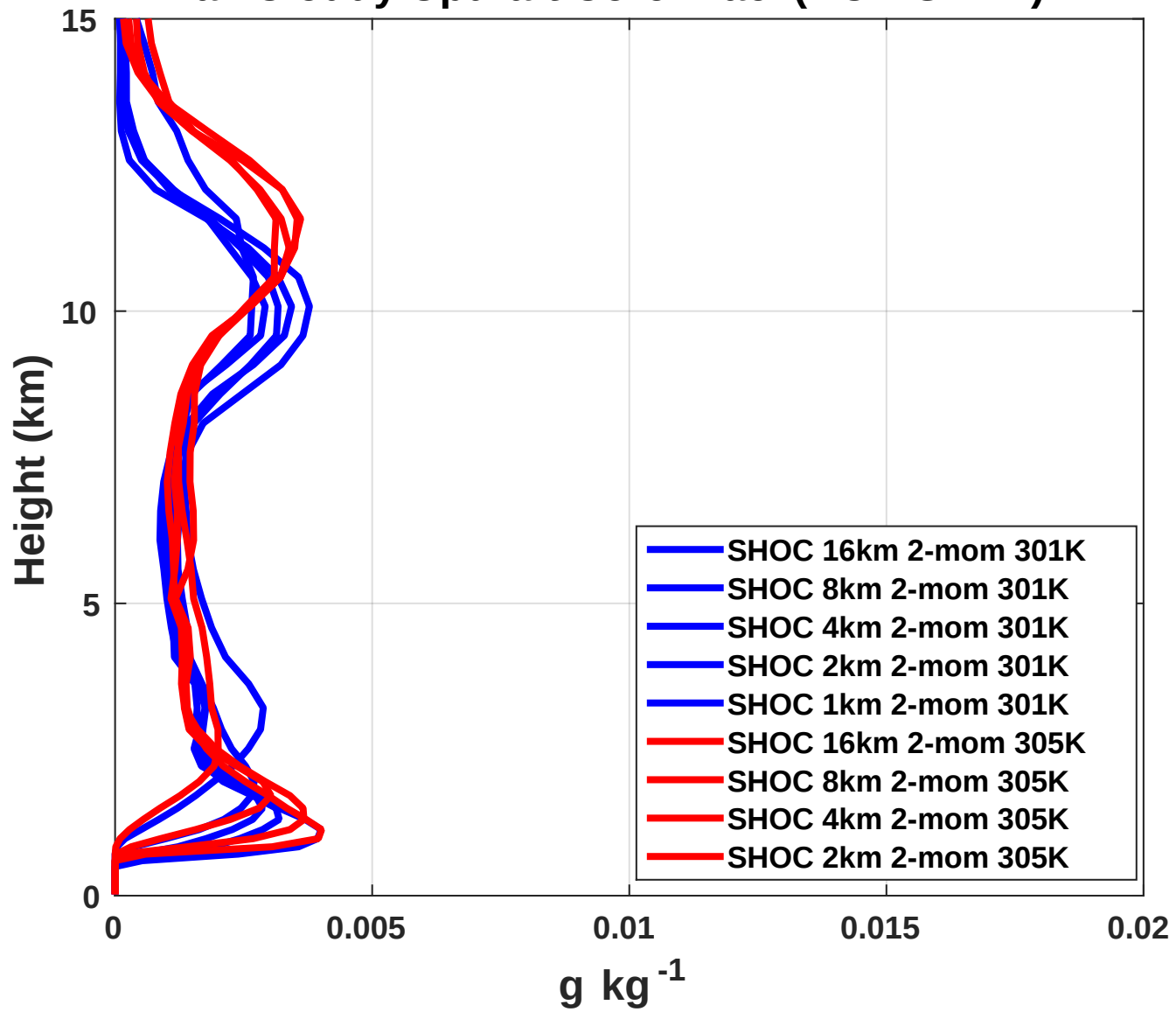
Max Cloudy Updraft Core Frac. (RCE-GREY)
