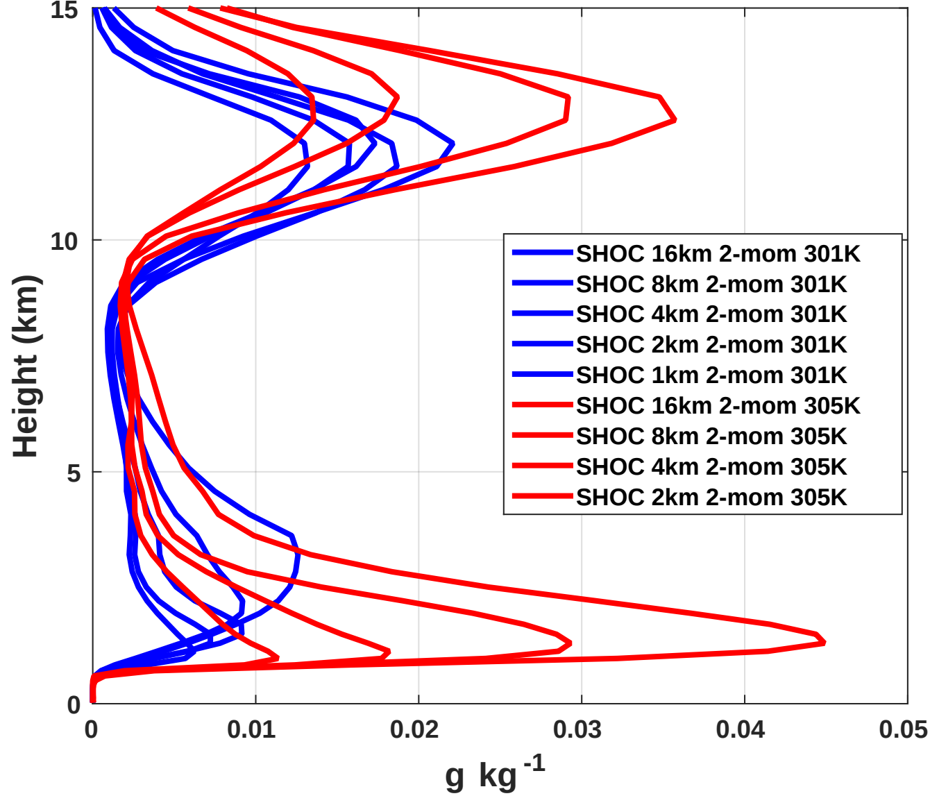
Total Cloud Condensate (RCE-GREY)
