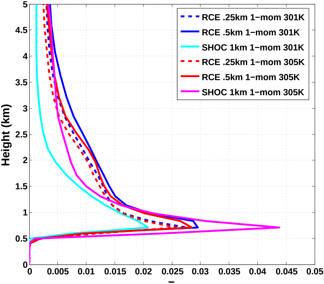
Cloud Fraction (RCE-GREY)
