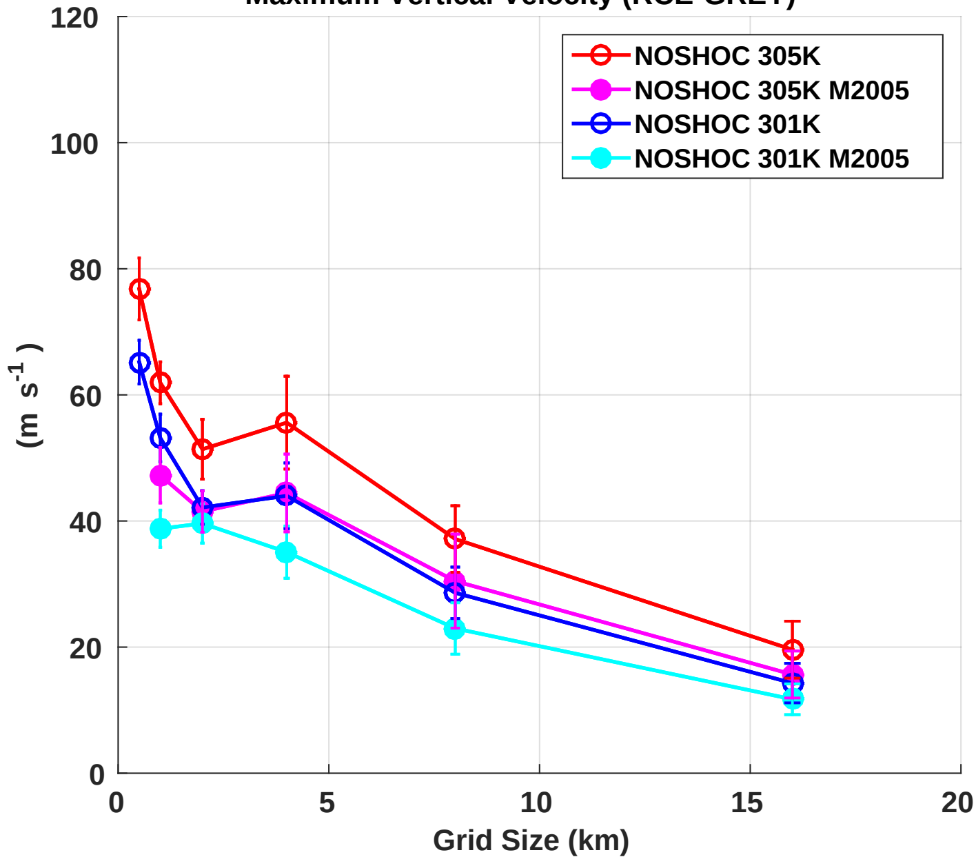
Maximum Vertical Velocity (RCE-GREY)
