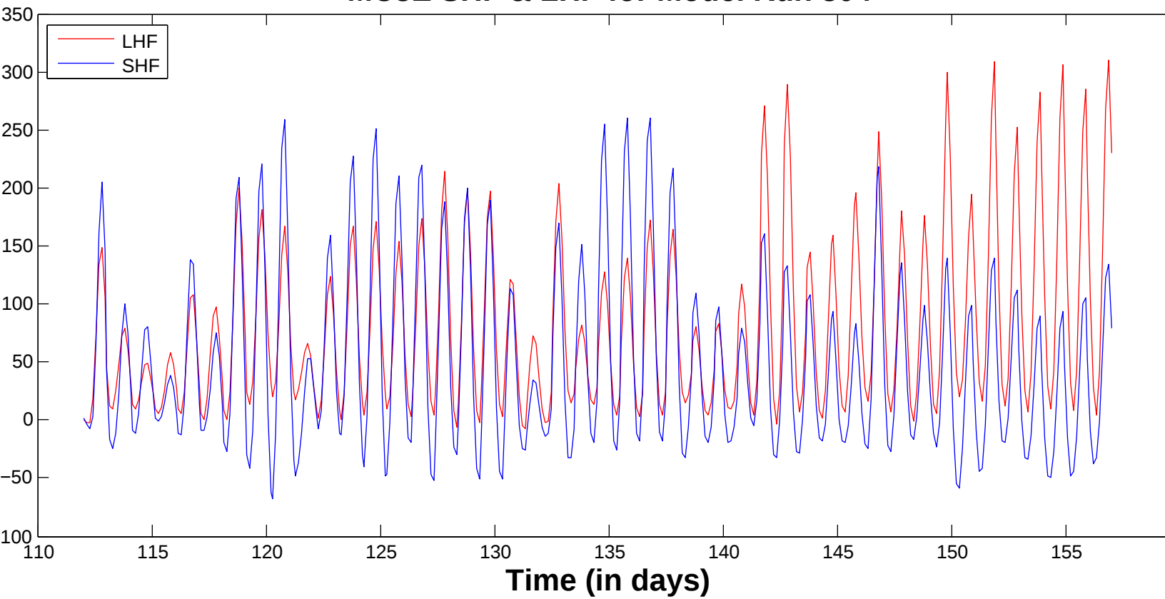
MC3E SHF & LHF for Model Run 304
