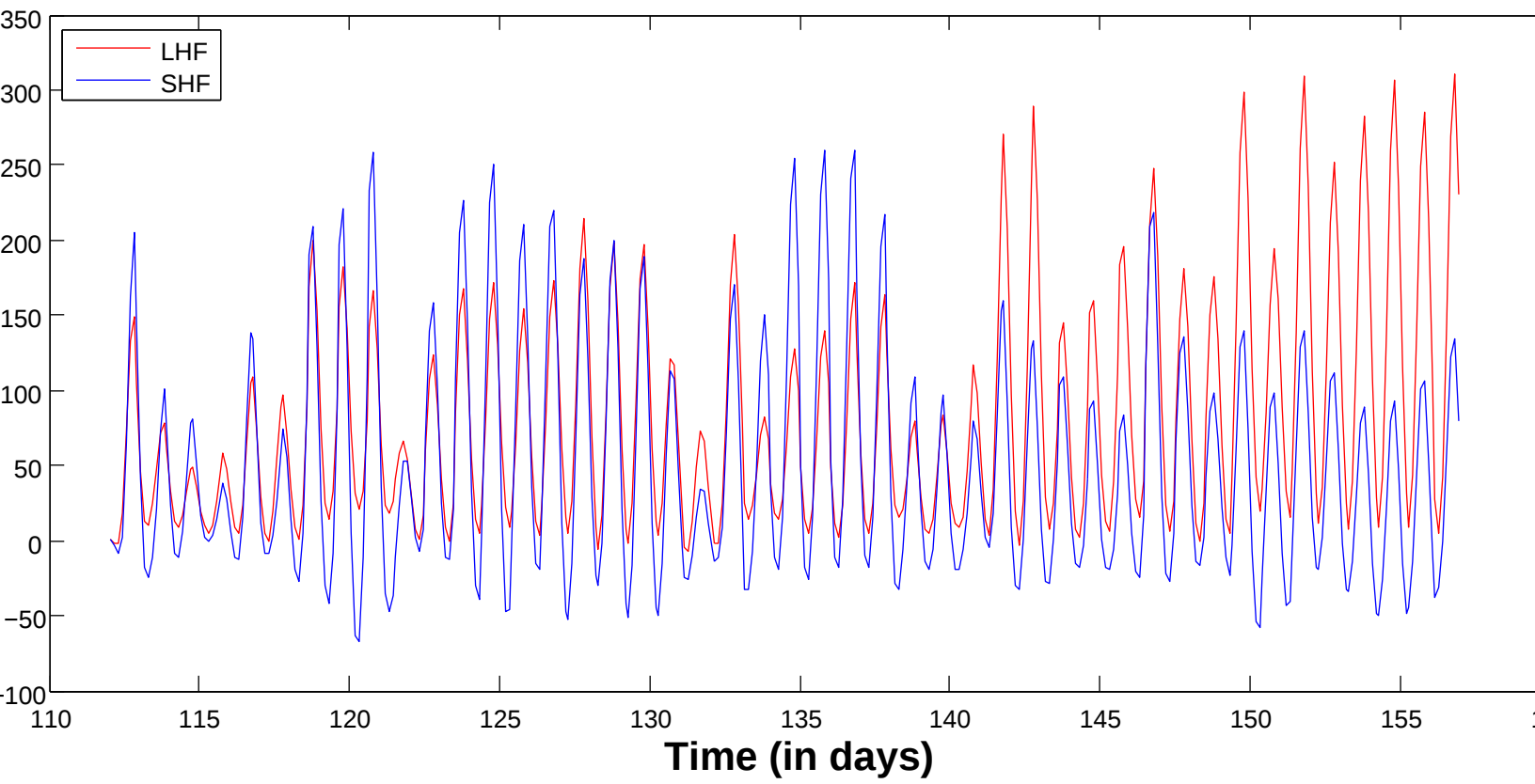
MC3E SHF & LHF for Model Run 306
