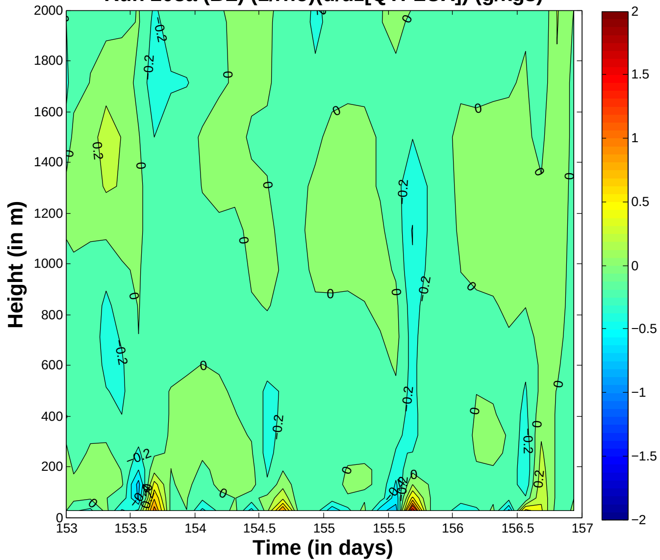
Run 208a (BL) (1/\rho)(d/dz[QTFLUX]) (g/kgs)
