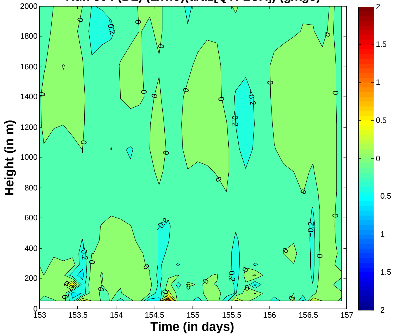
Run 304 (BL) (1/\rho)(d/dz[QTFLUX]) (g/kgs)
