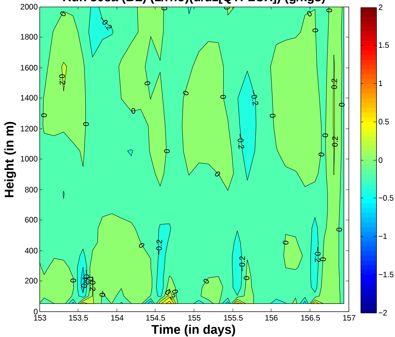
Run 308a (BL) (1/\rho)(d/dz[QTFLUX]) (g/kgs)
