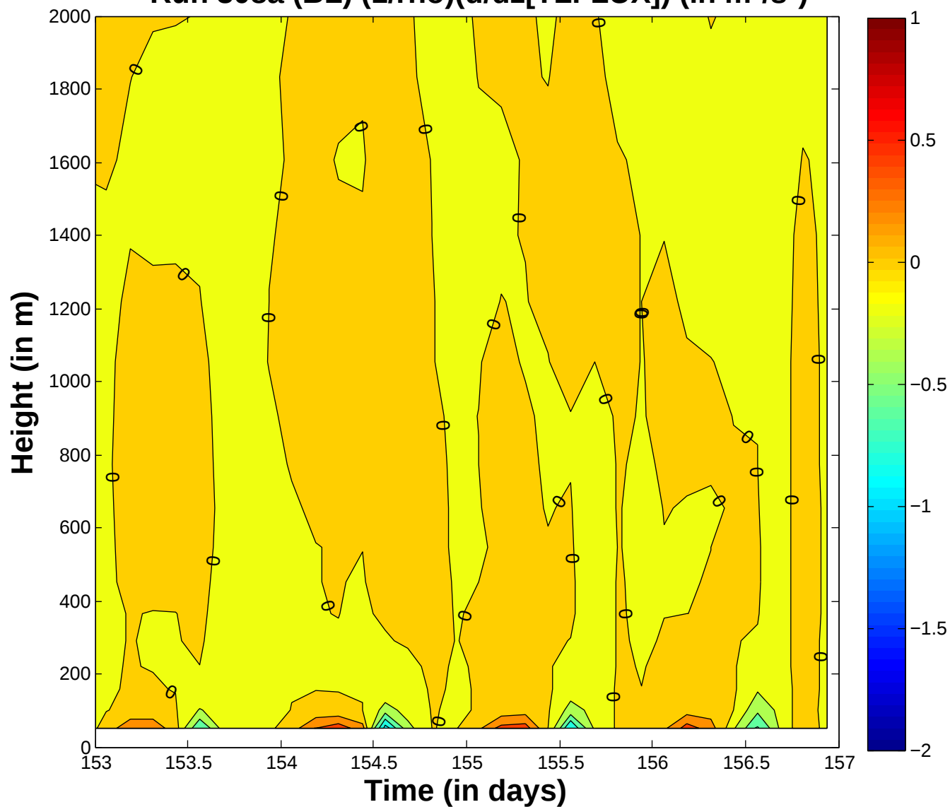
Run 308a (BL) (1/\rho)(d/dz[TLFLUX]) (in m^2/s^3 )
