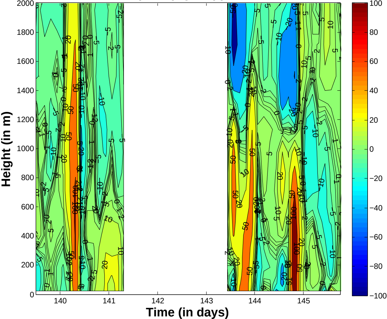
Run 208b & 208a (Conv) Q2: Apparent moisture sink
