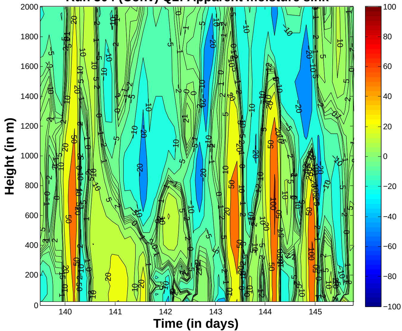
Run 304 (Conv) Q2: Apparent moisture sink
