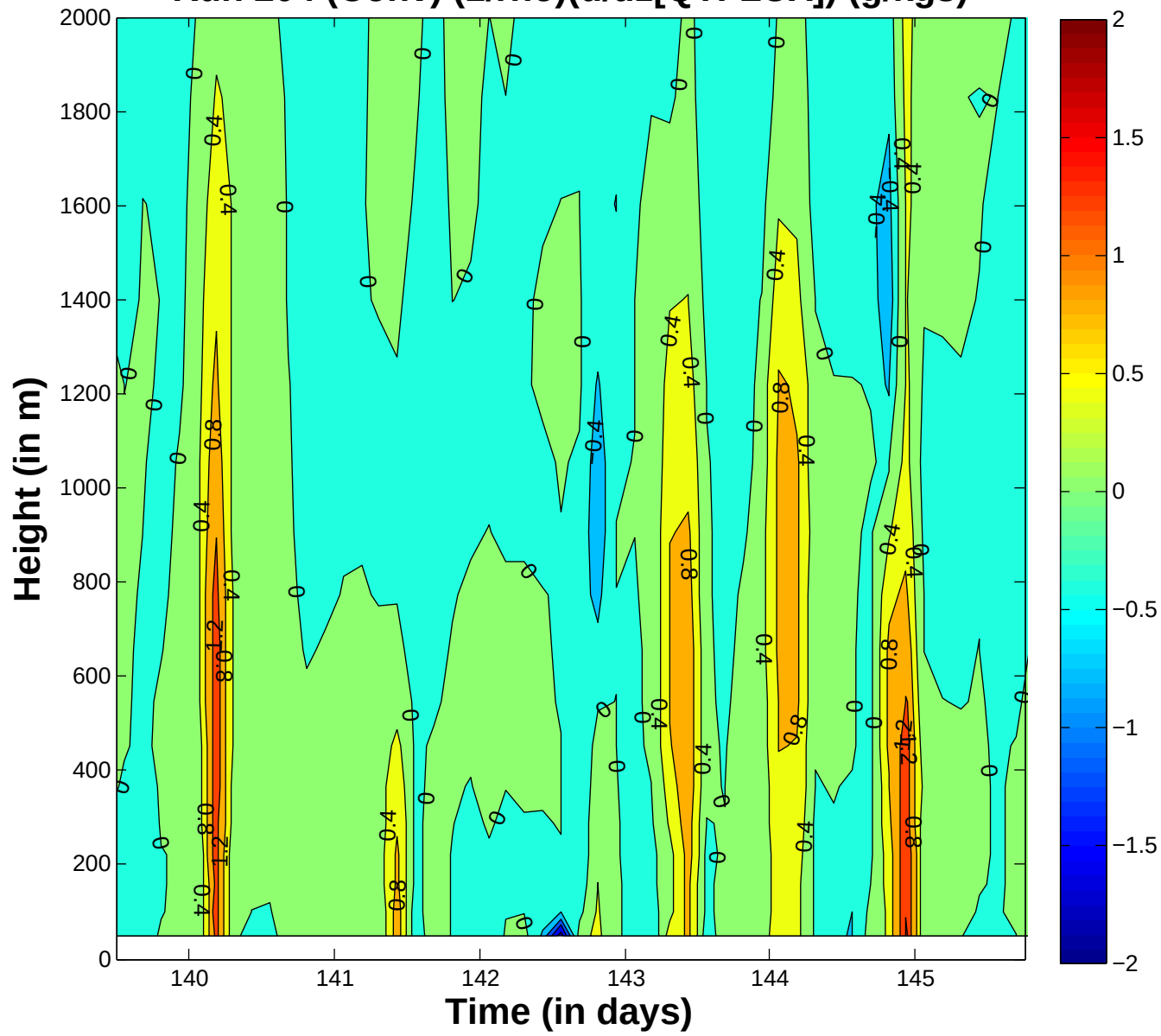
Run 204 (Conv) (1/\rho)(d/dz[QTFLUX]) (g/kgs)
