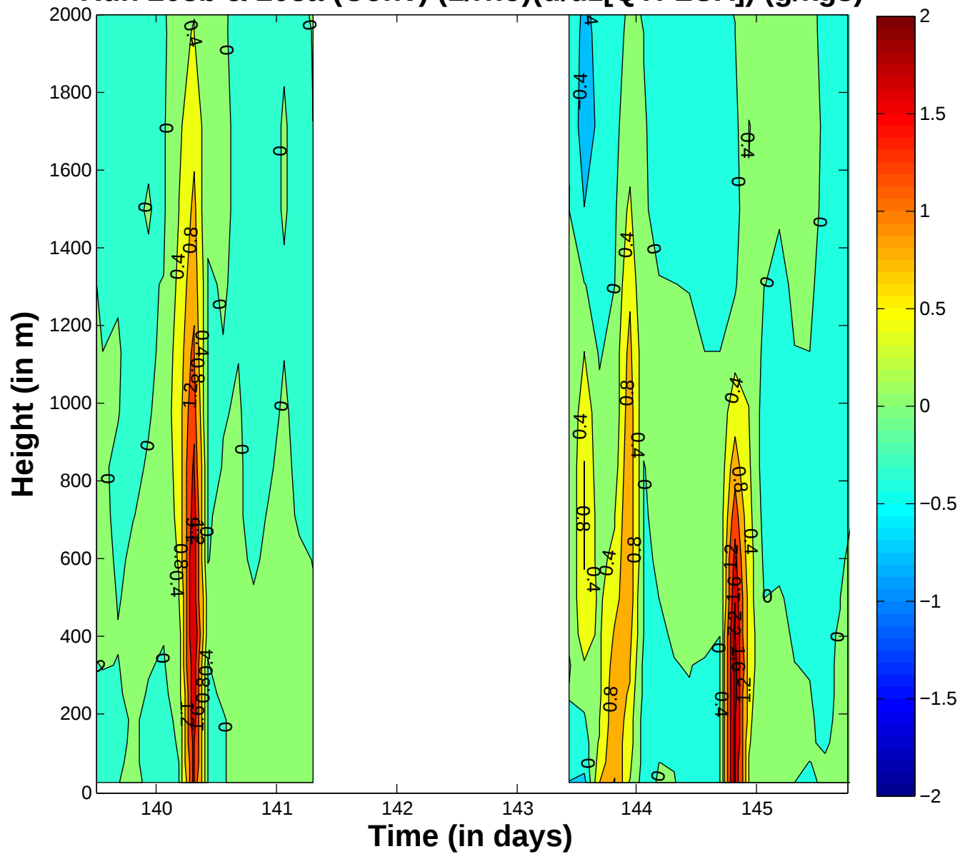
Run 208b & 208a (Conv) (1/\rho)(d/dz[QTFLUX]) (g/kgs)
