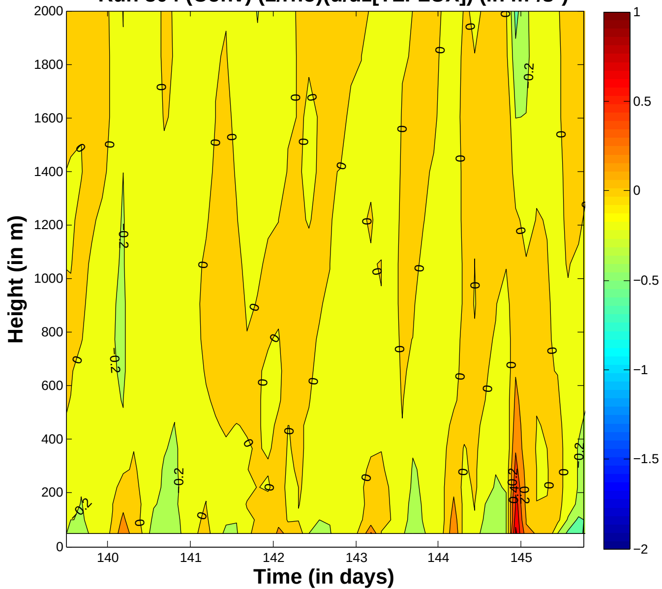
Run 304 (Conv) (1/\rho)(d/dz[TLFLUX]) (in m^2/s^3 )
