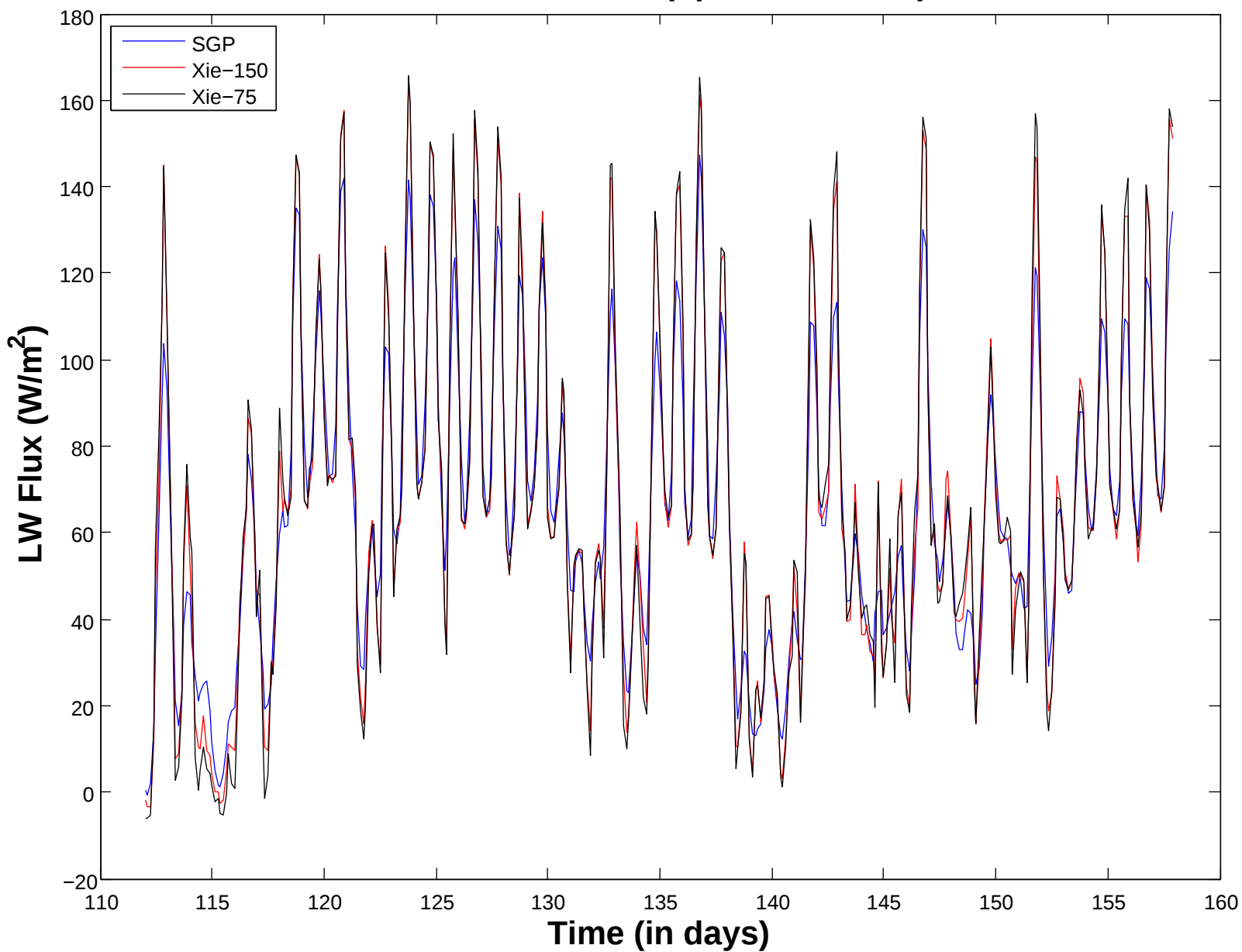
Surface LW Flux (up minus down)
