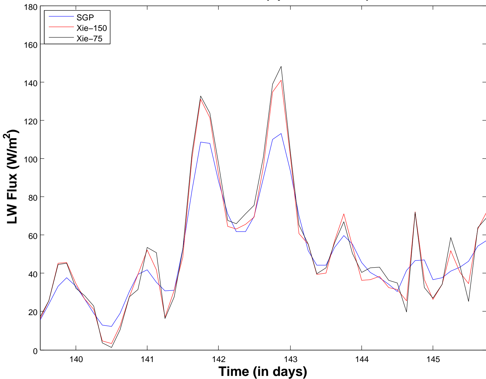
Surface LW Flux (up minus down)
