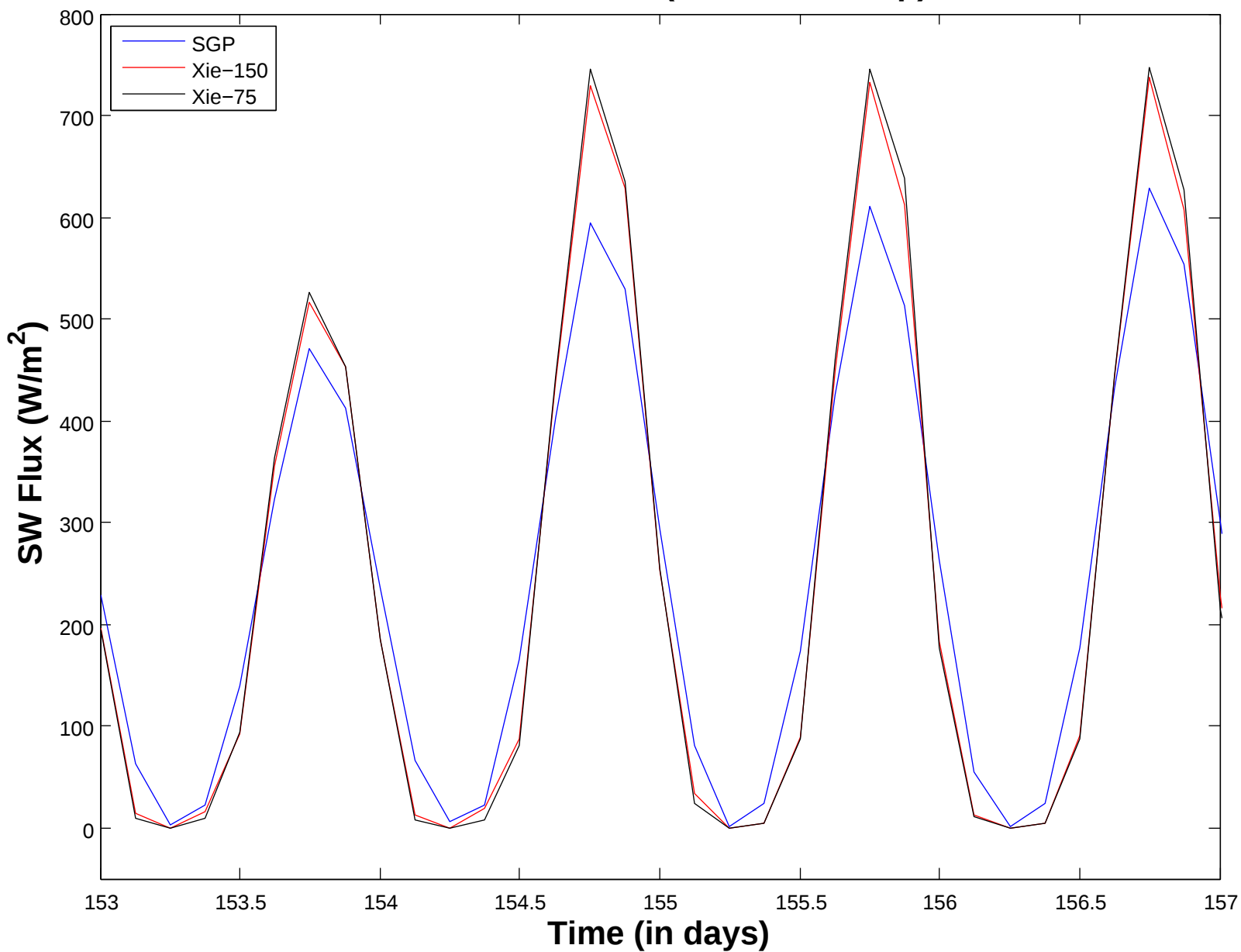
Surface SW Flux (down minus up)
