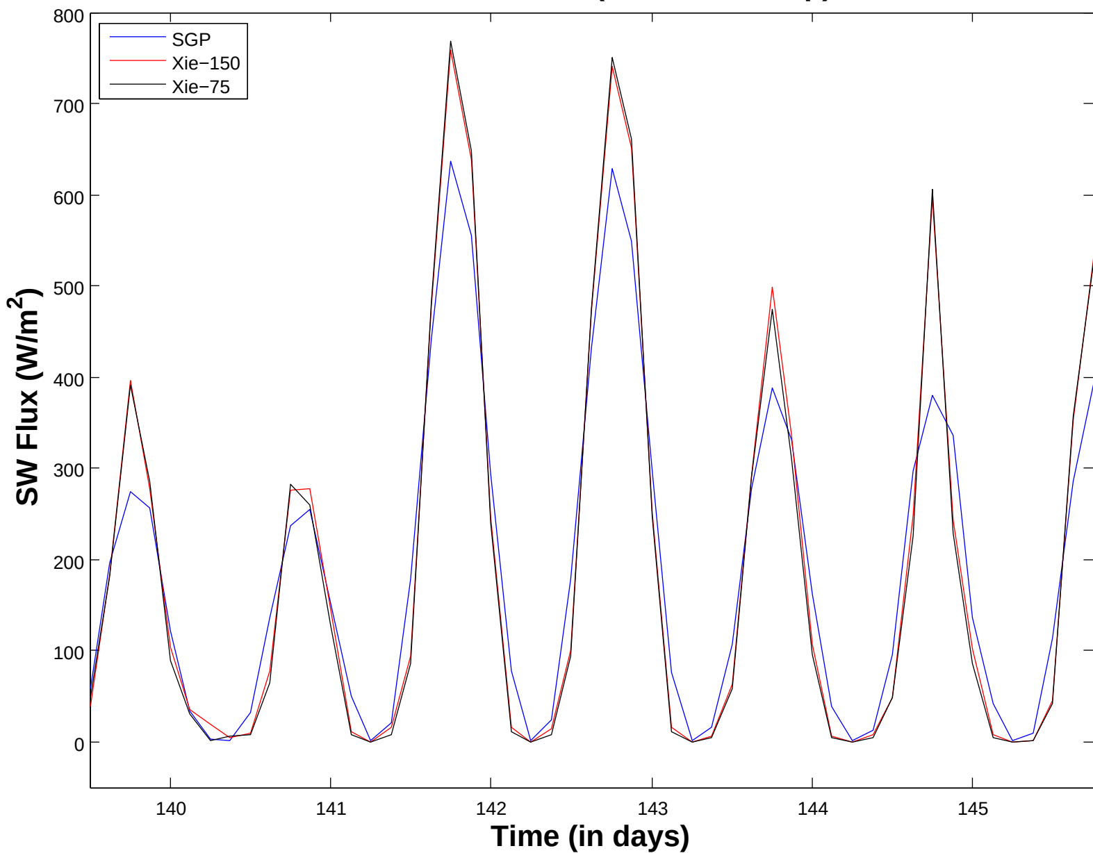
Surface SW Flux (down minus up)
