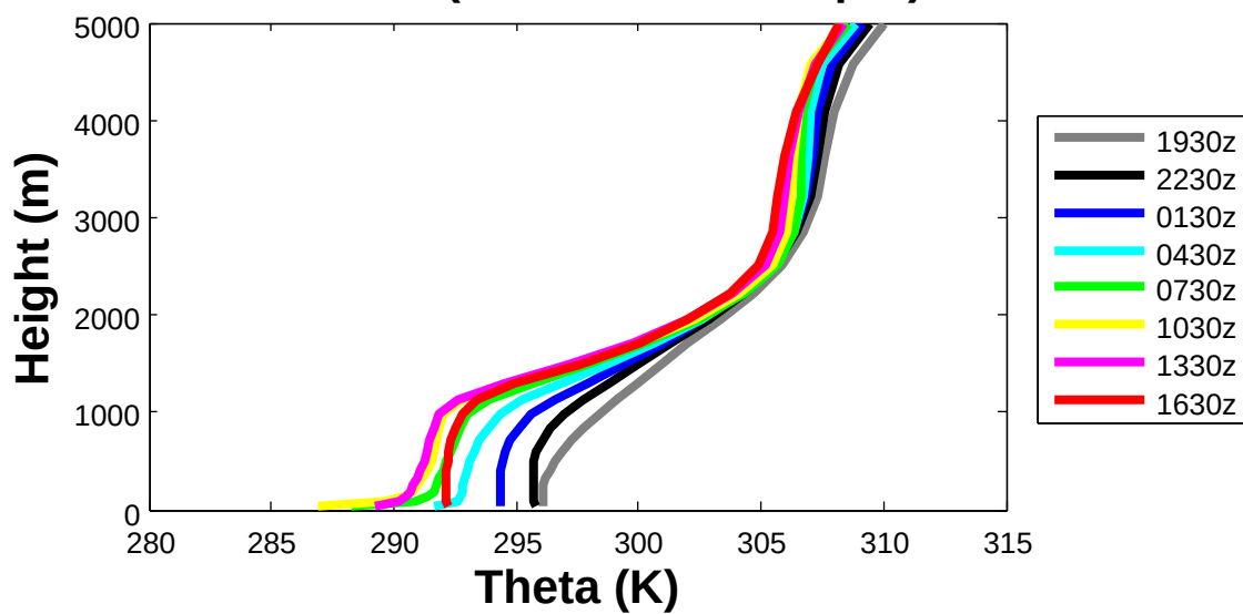
MC3E \Theta Profiles (18z–18z 25–26 April) Run 306
