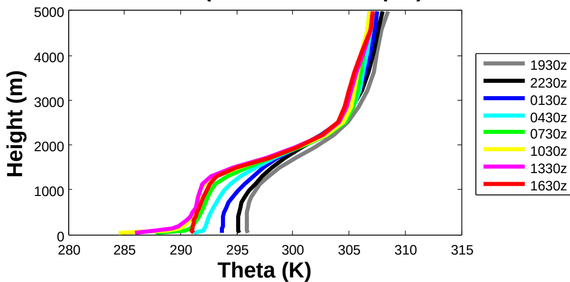
MC3E \Theta Profiles (18z–18z 25–26 April) Run 304
