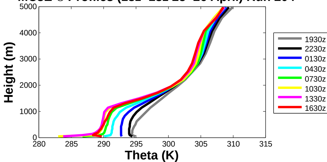
MC3E \Theta Profiles (18z–18z 25–26 April) Run 204
