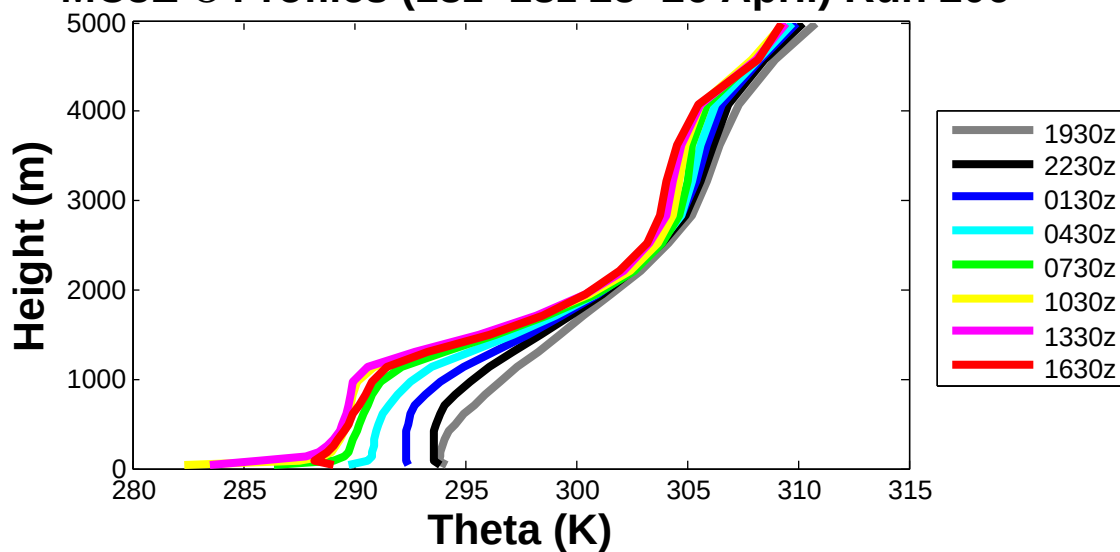
MC3E \Theta Profiles (18z–18z 25–26 April) Run 206
