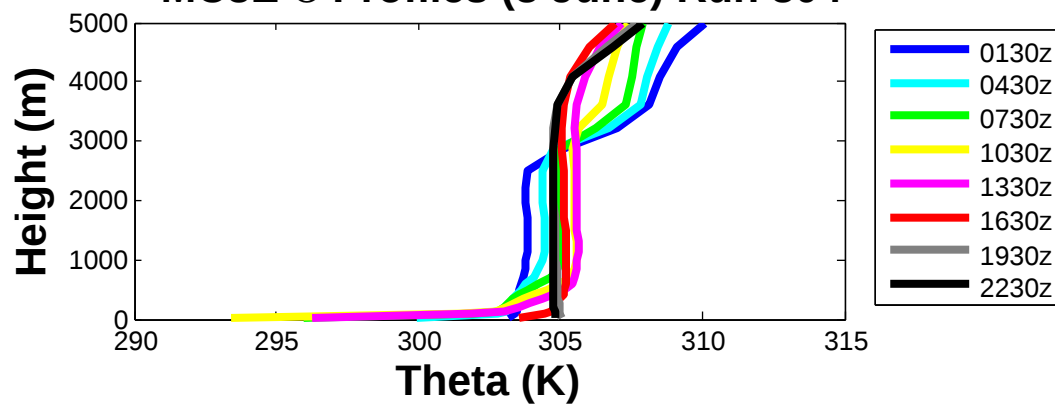
MC3E \Theta Profiles (3 June) Run 306
