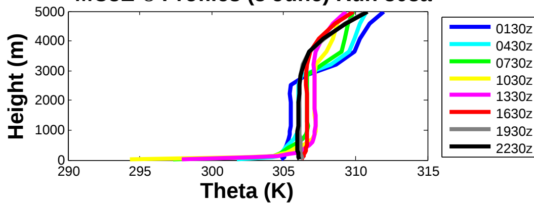
MC3E \Theta Profiles (3 June) Run 308a
