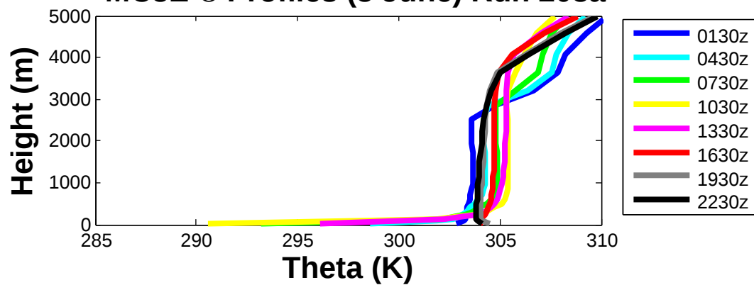
MC3E \Theta Profiles (3 June) Run 208a
