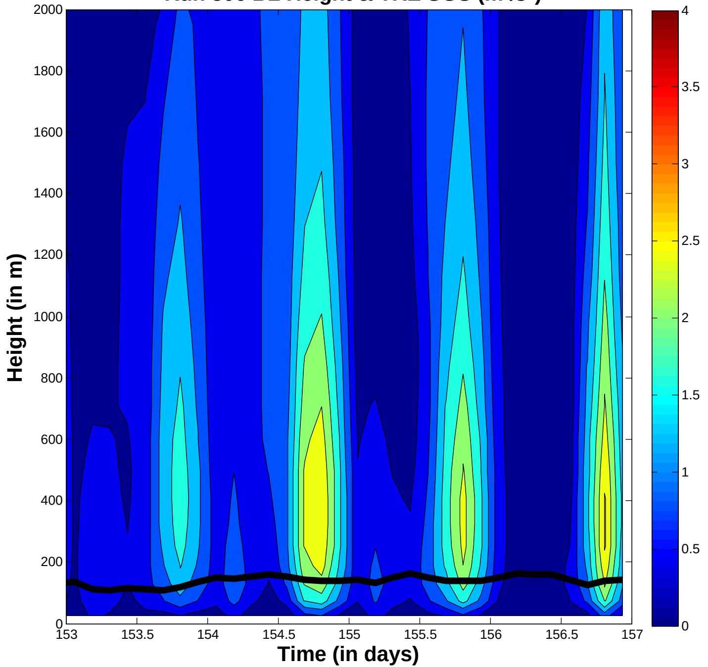
Run 306 BL Height & TKE SGS ( \text{m}^2/\text{s}^2 )
