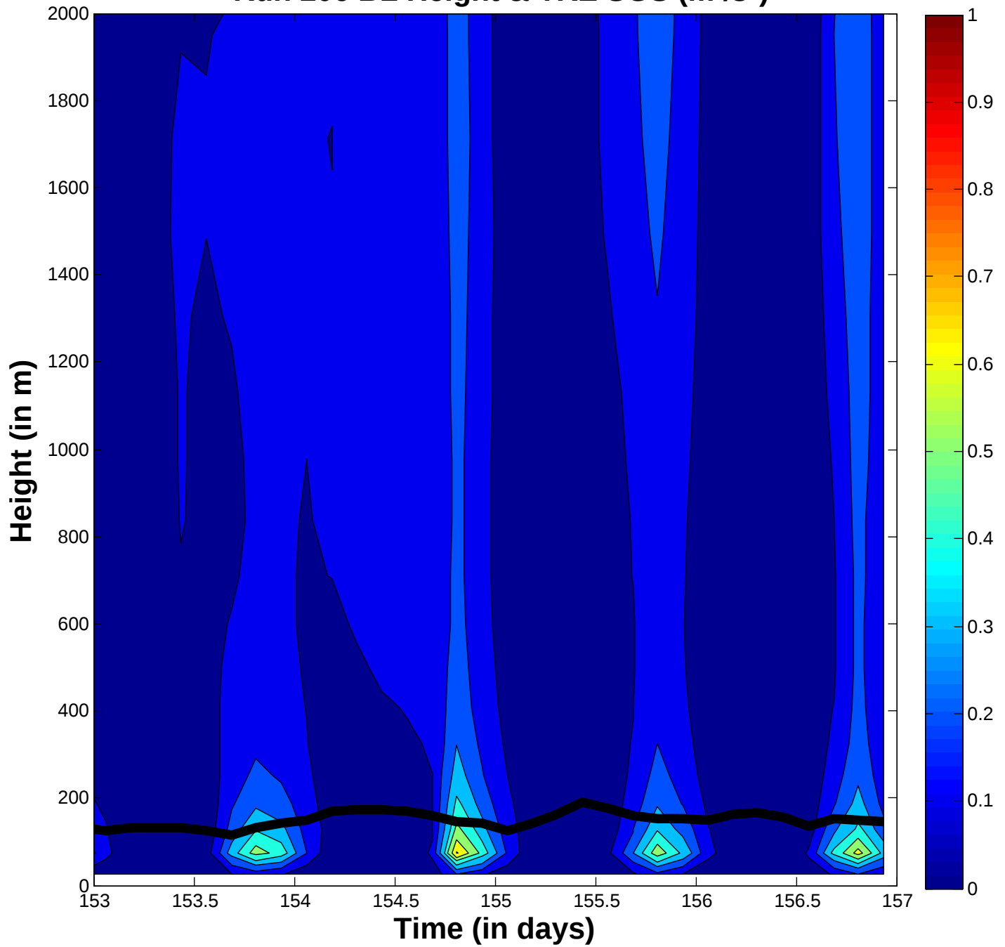
Run 206 BL Height & TKE SGS ( \text{m}^2/\text{s}^2 )
