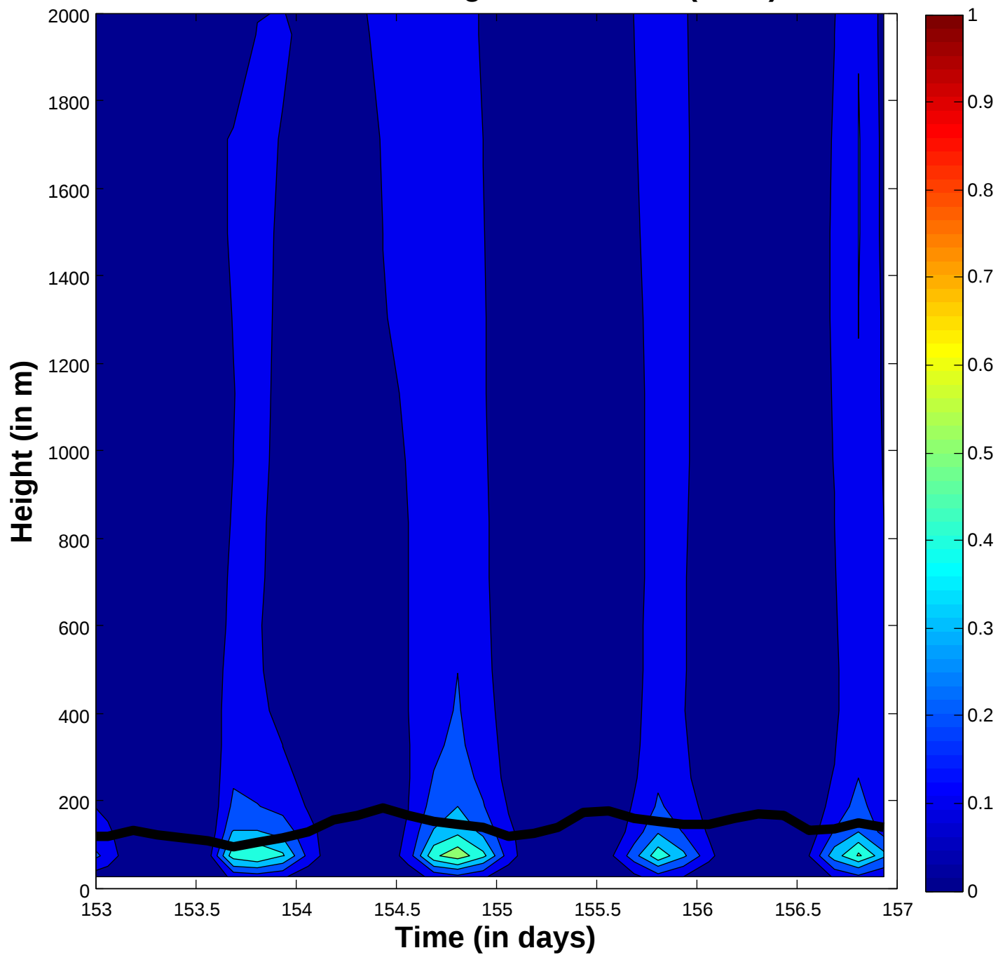
Run 208a BL Height & TKE SGS ( \text{m}^2/\text{s}^2 )
