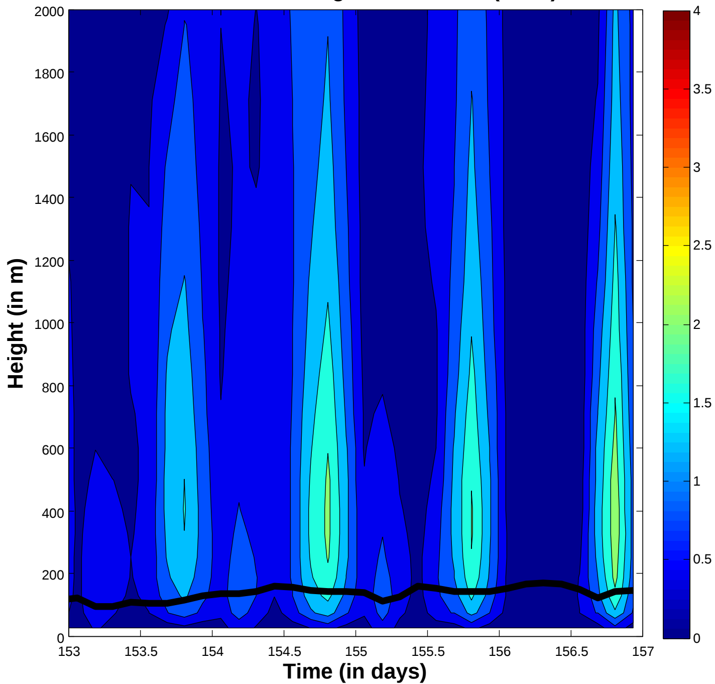
Run 308a BL Height & TKE SGS ( \text{m}^2/\text{s}^2 )
