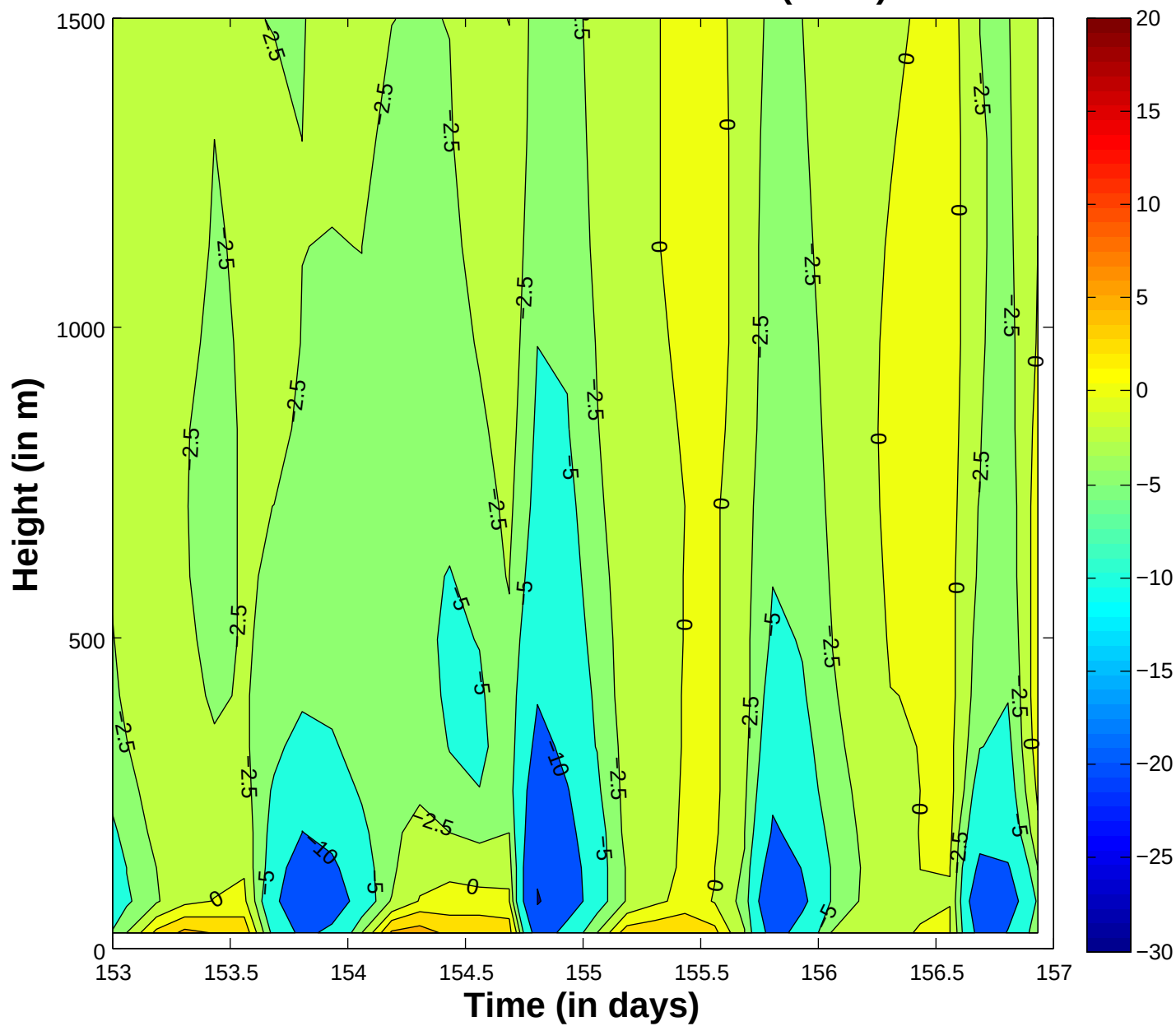
Run 304 – 204 TKE Resolved ( \text{m}^2/\text{s}^2 )
